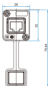
SX socket ( dimensions figure )
