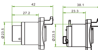
SX socket ( dimensions figure )
