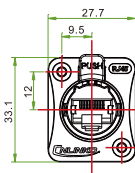
SX socket ( dimensions figure )
